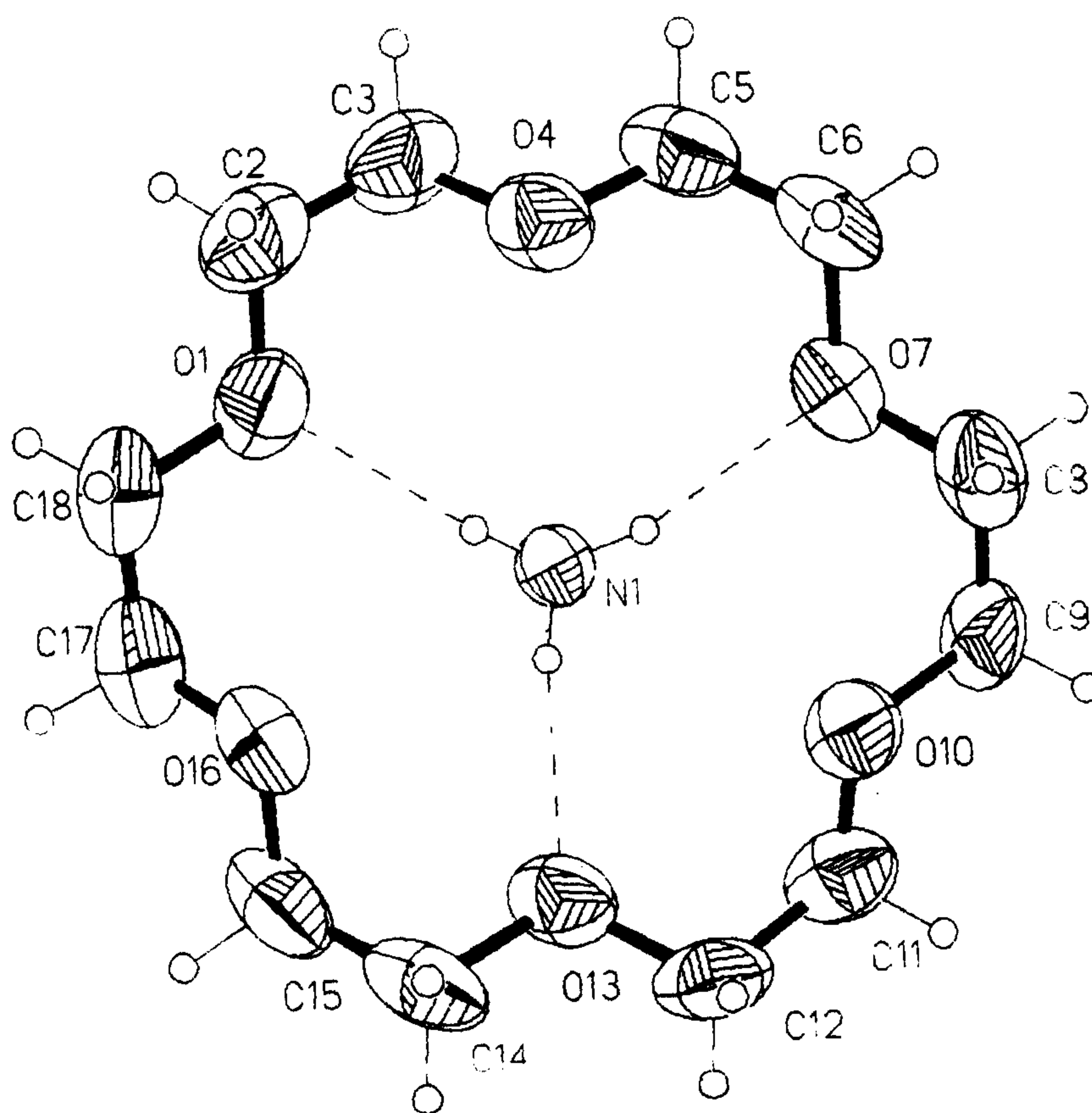
Figure 1. The view of the complex [\text{NH}_4 \cdot 18\text{C}6]^+ cation with the atom labelling and hydrogen bonds as dotted lines. The thermal ellipsoids are given with the 50% probability.
