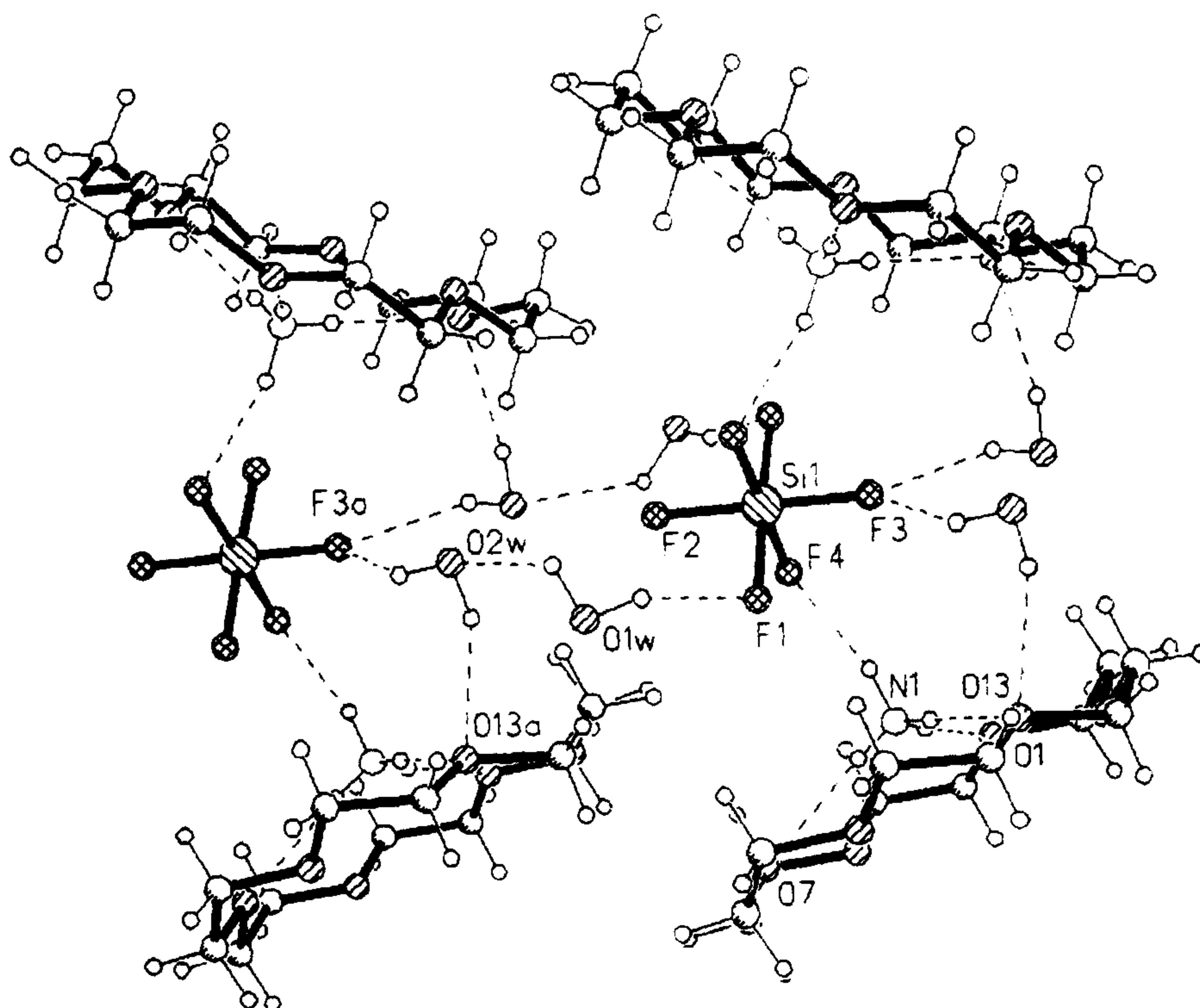
Figure 2. Packing diagram for the complex [(18\text{-crown-}6 \cdot \text{NH}_4)_2][\text{SiF}_6] \cdot 4\text{H}_2\text{O} .
